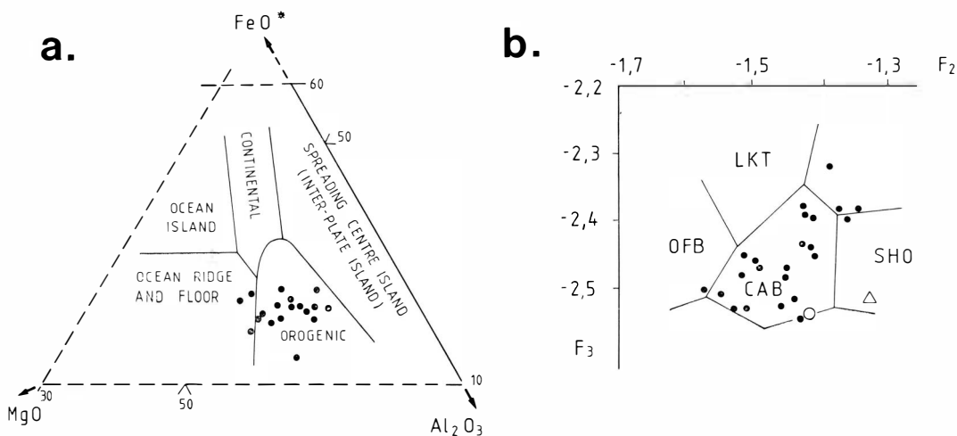
Fig. 7 (a). Part of the MgO-FeO*-Al 2 O 3 diagram of Pearce et al. (1977) showing the distribution of screened samples of Smöla volcanites. The samples are those with 50-56 wt.% SiO 2 , volatile-free. The 'orogenic' field embraces island arcs and continental margins. (b). Plot of major element discriminant functions, F 2 vs. F 3 (after Pearce (1976)) for the Smöla basalts and basaltic andesites. Only screened samples are used; for selection procedure see Pearce (1976). For comparison purposes the mean values for the Smöla andesites (open circle) and Holönda andesites (triangle) (Loeschke 1976a) are also plotted. The fields shown are as follows: CAB — calc-alkaline basalts; LKT — low-K tholeiites; OFB — ocean-floor basalts; SHO — shoshonites.
