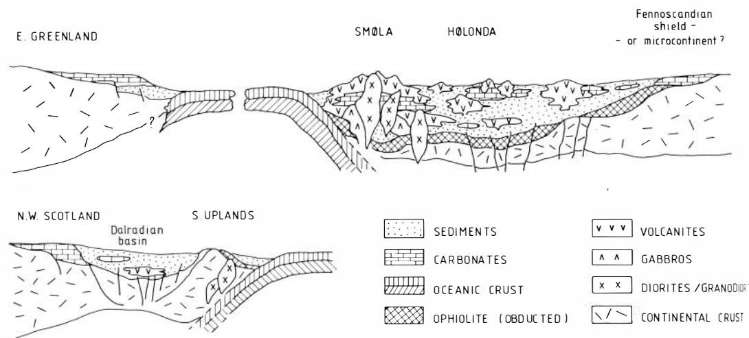
Fig. 9. Schematic, composite reconstruction of the suggested palaeogeographic/plate tectonic situation in Llanvirnian (-Caradocian) time to show the position of the mature Smøla arc in relation to the Hølonða area and the Ordovician back-arc basin of the Trondheim region. In this sketch the deepening basin east of Smøla is emphasized at the expense of the slightly earlier, Arenig-early Llanvirn fault troughs of the Hølonða area (cf. Bruton & Bockelie 1980), and the uplifted areas of 'continental' rocks to the east (cf. Ryan et al. 1980). The East Greenland continental margin with shallow-shelf limestones is also indicated. The Iapetus Ocean, between Greenland and Smøla, is purposely foreshortened in this diagram. The smaller sketch (lower left) shows the general situation in the British orthotectonic segment of the orogen on the W-NW side of Iapetus (modified from Phillips et al. (1976)). The diagram is not drawn to scale.
