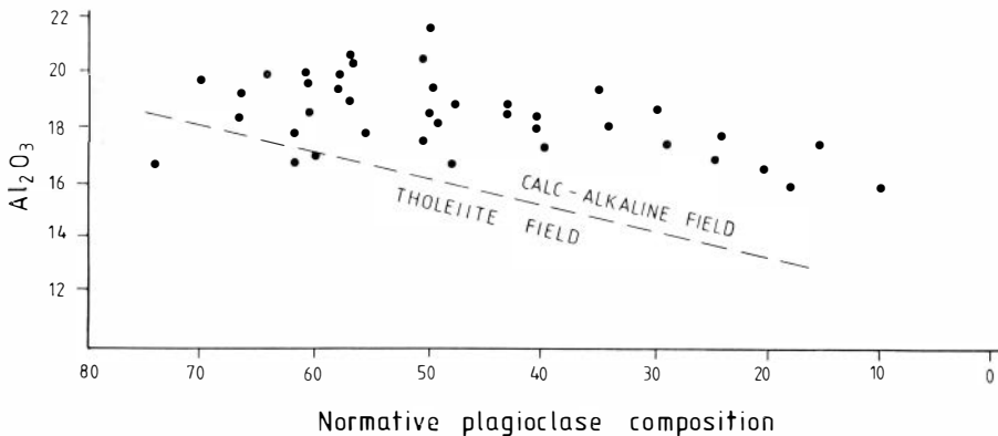
Fig. 6. The Smøla volcanic rocks on a plot of wt.% Al_2O_3 vs. normative plagioclase. The dividing line between the calc-alkaline and tholeiite fields is from Irvine & Baragar (1971).
