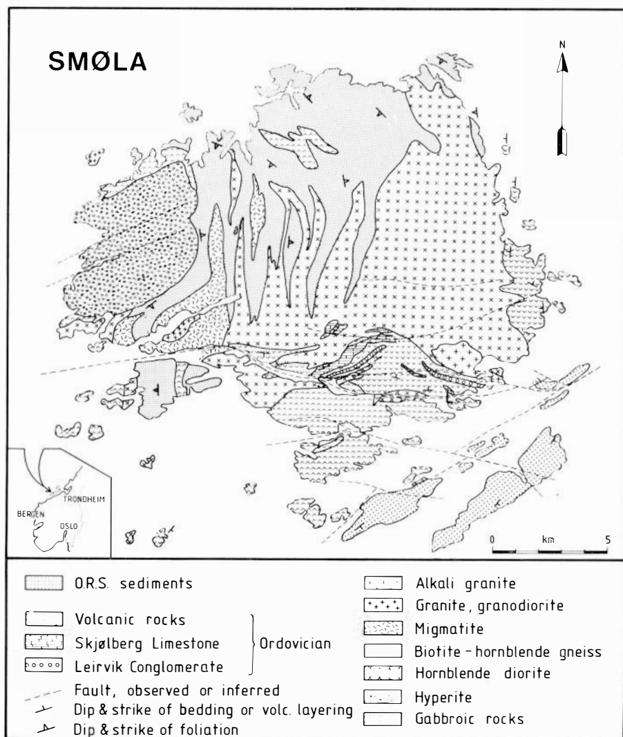
Fig. 1. Simplified geological map of Smøla. The geology is from Fediuk (1975) with minor amendments after Bruton & Bockelie (1979) and the author. S - Skjølberg. L - Leirvik.
