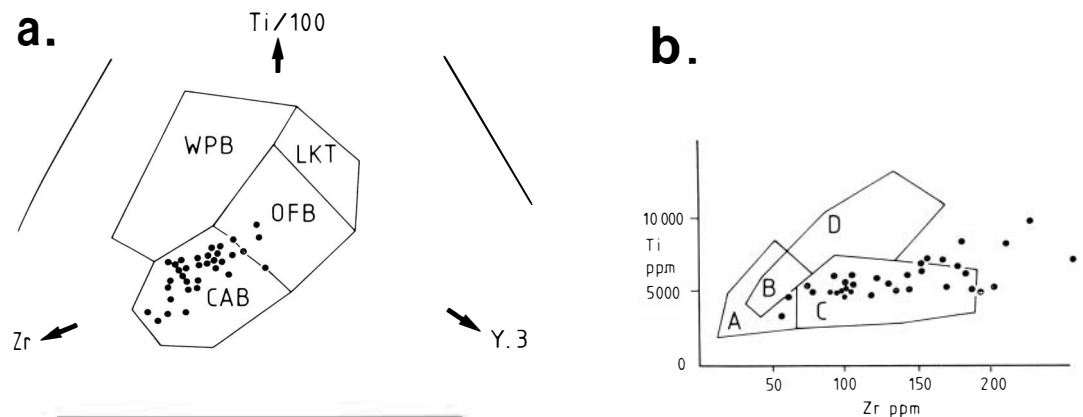
Fig. 8 (a). Smöla basalts and andesites plotted on the Ti-Zr-Y discrimination diagram of Pearce & Cann (1973). CAB — calc-alkaline basalts; OFB — ocean floor basalts; LKT — low-K tholeiites; WPB — within-plate basalts. (b). Ti vs. Zr variation for the Smöla basalts and andesites; after Pearce & Cann (1973). Fields A+B — low-K tholeiites; C+B — calc-alkali basalts; D+B — ocean floor basalts.
